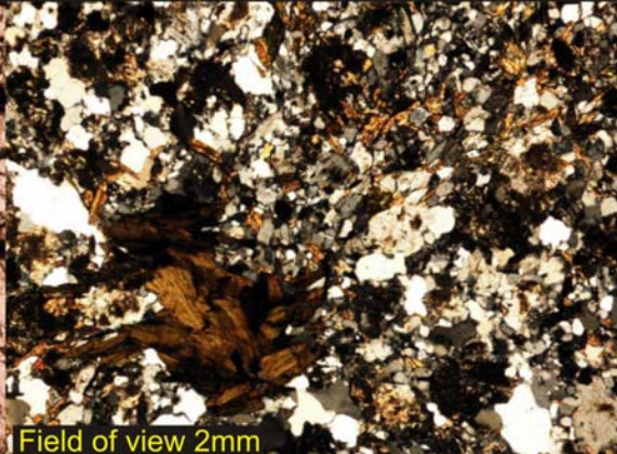
Gneiss xpl
