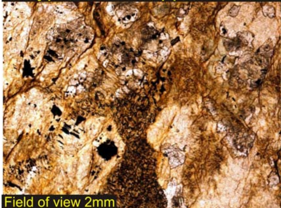
Polyphant stone ppl
