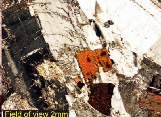
Coarse grained granite xpl
